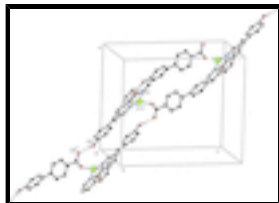
Fig. 2. Partial packing view showing the formation of the chain through O-H...O hydrogen bonds which are shown as dashed lines. H atoms not involved in hydrogen bondings have been omitted for clarity. [Symmetry code: (i) x-1/2, -y+3/2, z-1/2 ]
